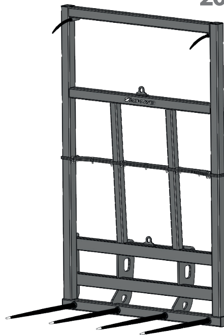
PIC BALLE AP 2001 4 DENTS Ø45 LG 1055 PERCEE
