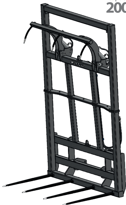
PIC BALLE AP 2000 4 DENTS Ø45 LG 1200 PERCEE
