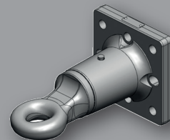
BOLT-ON SWIVEL HITCH EYE 145X145 448048 E.U. HOMOLOGATED 2018/829
