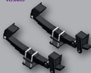
1/2 TANDEM SET 6 BLADES 448166 Available in multi-leaf and parabolic versions
